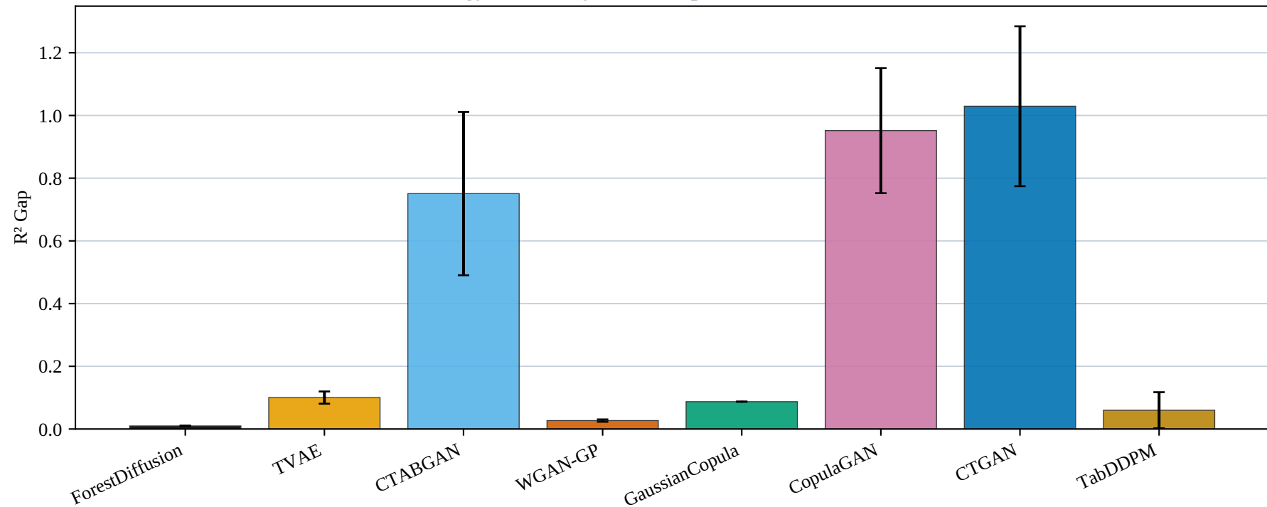
Energy Efficiency — R^2 Gap (mean \pm SD, 10 seeds)
